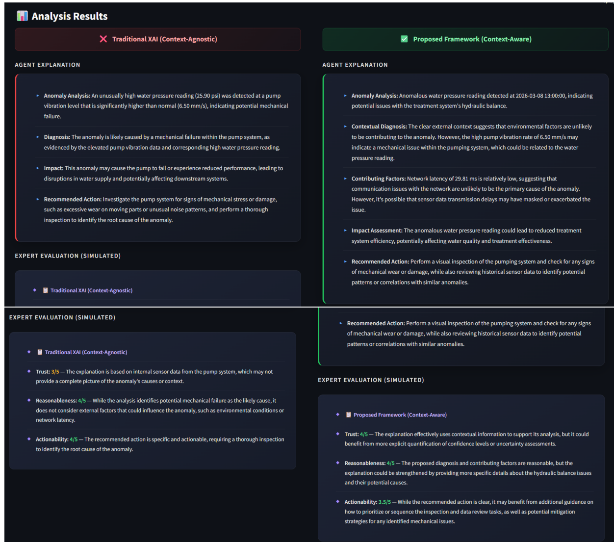
Figure 5: The multi-agent output interface. Top: Side-by-side empirical comparison contrasting traditional context-agnostic XAI with the proposed context-aware framework. Bottom: The automated LLM-as-a-Judge scorecards grading both explanations on Actionability, Reasonableness, and Trust.
